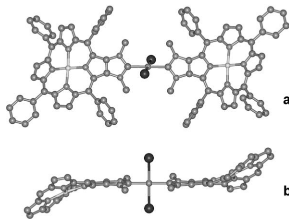
Fig. 2 Two views of the X-ray structure of the complex 10 (solvent molecules have been omitted for clarity). (a) t -Butyl groups and Hs omitted for clarity. (b) meso -Aryl groups and Hs omitted for clarity.
