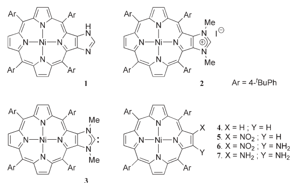
Fig. 1 Structures of the complexes 1–7.
